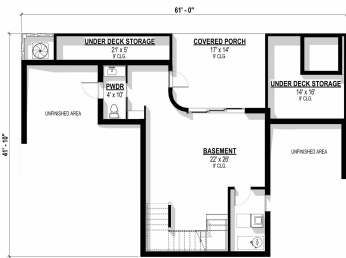
BASEMENT FLOOR PLAN
